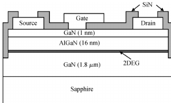
Figure 3. GaN HEMT Internal Structure [8]
