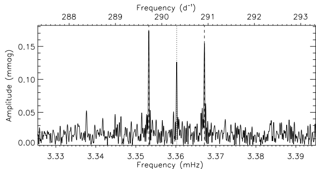
Figure C7. Amplitude spectrum for TIC 630844439. The vertical dotted line identifies the pulsation mode, with the dashed lines showing the rotational sidelobes.
