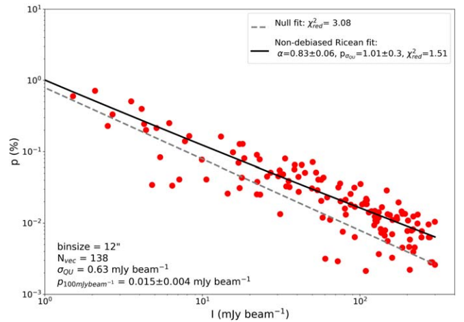
Figure 4. A plot of polarization fraction vs. Stokes I intensity of nondebaised polarization vectors in the inner 3' area of the map. The vectors are binned to 12'', and the only selection criteria is Stokes I > 0 . The null fit is plotted as a gray dashed line, while the Ricean fit is plotted as a black solid line. The \alpha value for the Ricean and reduced- \chi^2 values are given for both fits in the legend.
