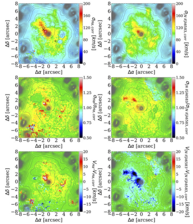
Figure 6. Comparison between fits using a single Gaussian and fits including a secondary [N II]\lambda 6583 component. Grey contours in all panels highlight the H\alpha emission. The left-hand and right-hand columns represent H\alpha and [N II]\lambda 6583 , respectively. Top: the corrected velocity dispersion ‘x’ and ‘+’ markers on the left-hand panel represent the spaxels whose spectra are displayed in Fig. 5. middle: The ratio of velocity dispersion obtained from single Gaussian fits to the corrected velocity dispersion. Bottom: The velocity differences between the corrected velocity field and the velocity field obtained with single Gaussians.
