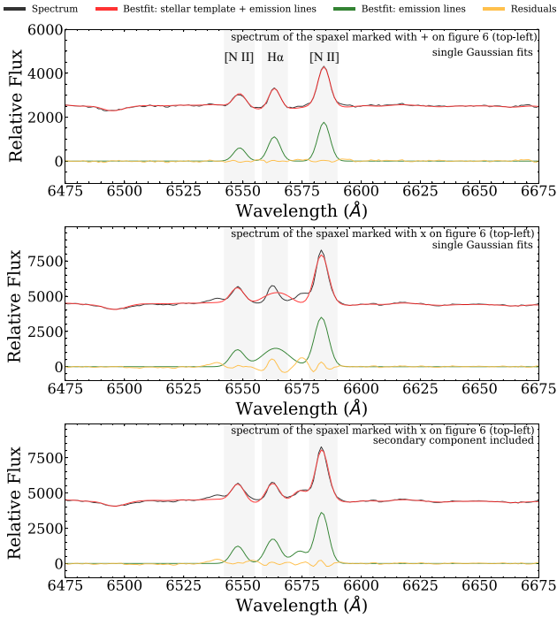
Figure 5. Representative spectra zoomed on the region of H\alpha and [N II]\lambda 6583 , and the best fits from pPXF/DAP. The lines represent the MUSE spectrum (black), the combined best fit of the stellar template and emission lines (red), the best fit of emission lines (green), and the difference between the spectrum and the combined best-fitting stellar template with emission lines (orange). top: Spectrum of a spaxel without the excess, marked in the upper left-hand panel of Fig. 6 with a ‘+’. middle: Spectrum of a spaxel with the excess affecting the single Gaussian fits of H\alpha and [N II]\lambda 6583 , marked in the upper left-hand panel of Fig. 6 with an ‘x’. bottom: Spectrum of the spaxel shown in the middle panel, with fits that include the secondary component.
