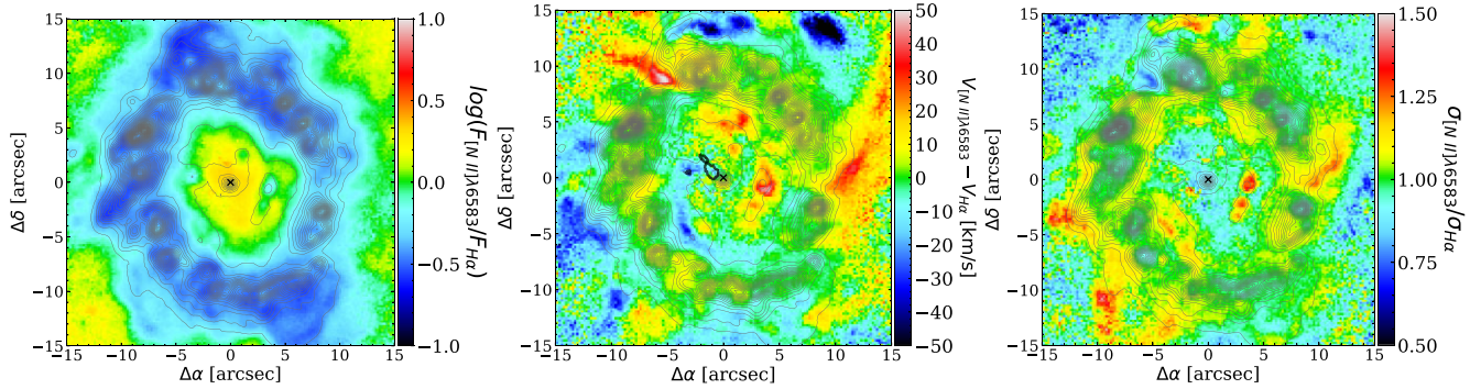
Figure 12. Left-hand panel: Line flux ratio of [N II]λ6583 and H \alpha . Middle: The velocity difference map, which is constructed by subtracting the LOS velocity of H \alpha from the LOS velocity of [N II]λ6583. Black contour marks the region where the velocity difference between [N II]λ6583 and H \alpha was more than 30 \text{ km s}^{-1} for single Gaussian fits. Right-hand panel: Velocity dispersion ratio of [N II]λ6583 and H \alpha . In all panels, grey contours highlight the H \alpha emission.
