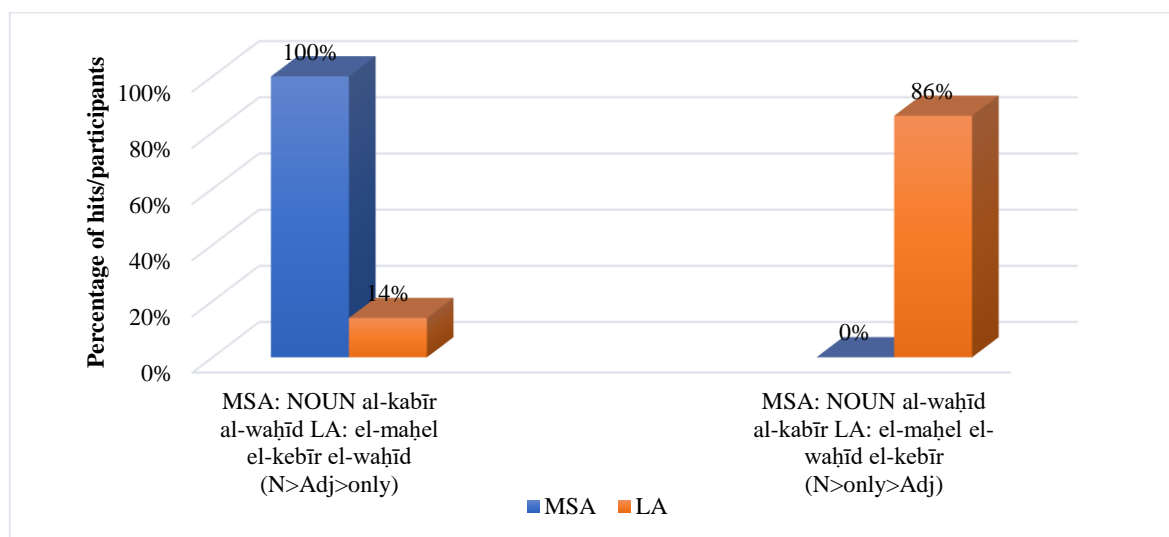
Figure 3. Specifying and Descriptive Adjectives
