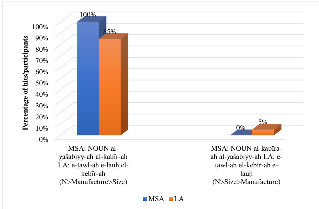
Figure 4. Manufacture and size adjectives
