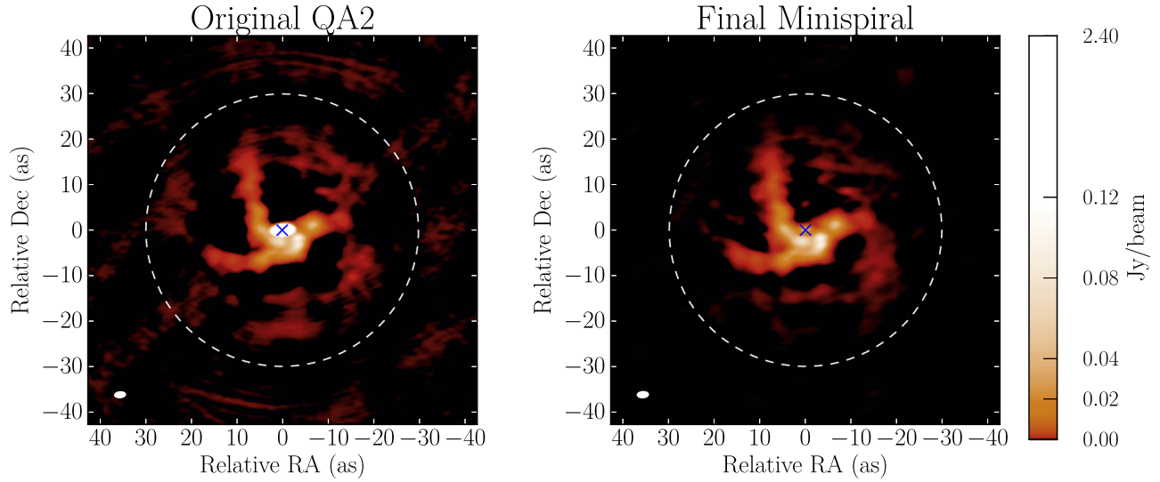
Figure 1. Left: an image of the Sgr A* field obtained from the original QA2 calibrated data, using natural weighting and a Gaussian taper in Fourier space to boost the sensitivity to the extended (minispiral) structure. Right: a final image of the minispiral, after applying the intrafield calibration and removing the signal from Sgr A*. In each panel, the convolving beam is shown in the lower left corner and the location of Sgr A* is marked with a cross. The dashed line marks the region where the primary-beam response of the ALMA antennas is above 5%.
