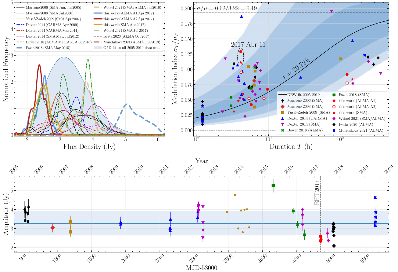
Figure 7. Top left: distributions of the published flux density measurements of Sgr A* at 230 GHz. Each distribution represents an epoch no longer than 16 days. Across all of the epochs, the flux density remained roughly within the 4 \pm 2 Jy range. Top right: modulation index, \sigma_T/\mu_T , measured in different observations as a function of the observation duration, T . The black median line and the 1\sigma , 2\sigma , and 3\sigma uncertainty bands, calculated with a Monte Carlo scheme, correspond to expectations from a damped random walk model fitted to the combined 2005–2019 data set (with the timescale \tau = 20.72 hr, and with the asymptotic modulation index of \sigma/\mu = 0.19 indicated with a dashed line; see also Section 5). Bottom: all data sets presented in Tables 1 and 6 with mean values and standard deviations indicated. The markers follow the convention of the top right panel. Additional points between 2013 and 2015 correspond to ALMA measurements reported in Bower et al. (2015). The horizontal line and blue bands correspond to the median value and 68% confidence interval of a GAD fit to combined 2005–2019 data sets.
