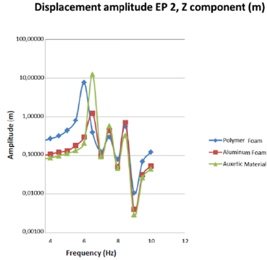
FIGURE 9. Amplitude-frequency graph for the three materials at point 2.
