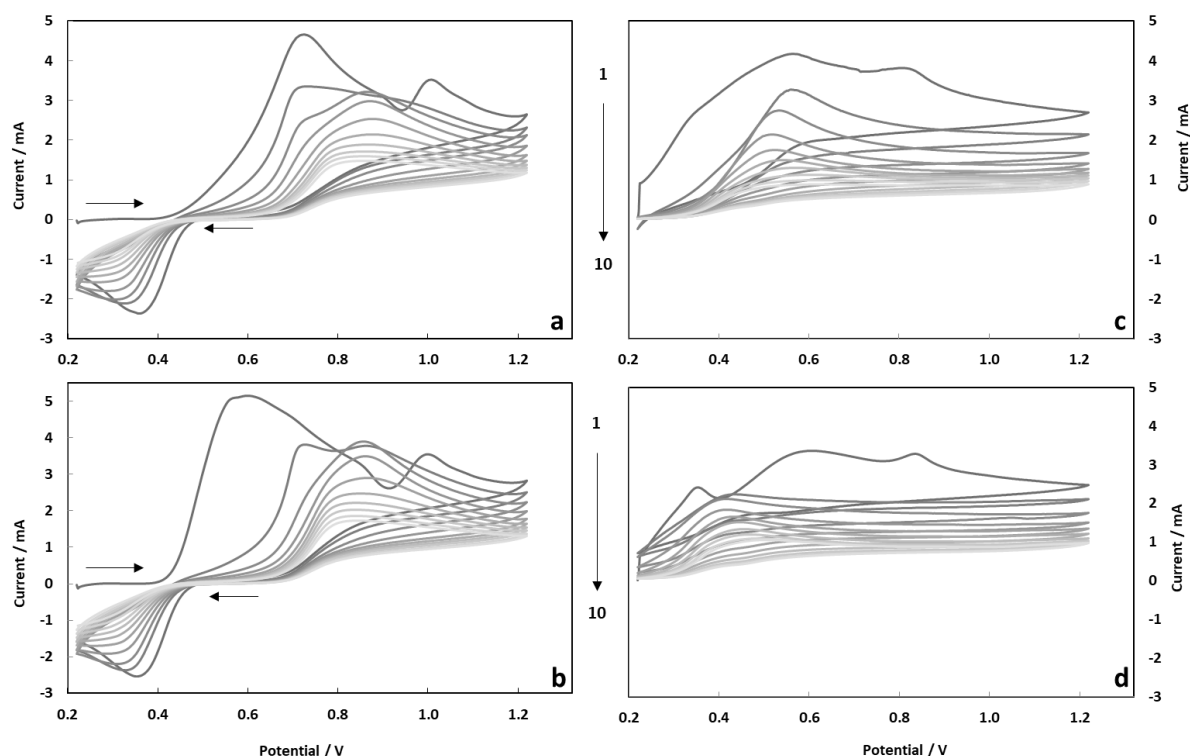
160 Fig.2 – CVs illustrating typical current responses in the 10 scan electropolymerisation process of 4-AP 161 in the presence of copper chloride for DOP MIP layers (a) and NIP layers (b); absence of copper 162 chloride DOP MIP layers (c) and NIP layers (d); all using \text{H}_2\text{SO}_4 (0.5 M) at a scan rate of 50 \text{ mV s}^{-1} .
