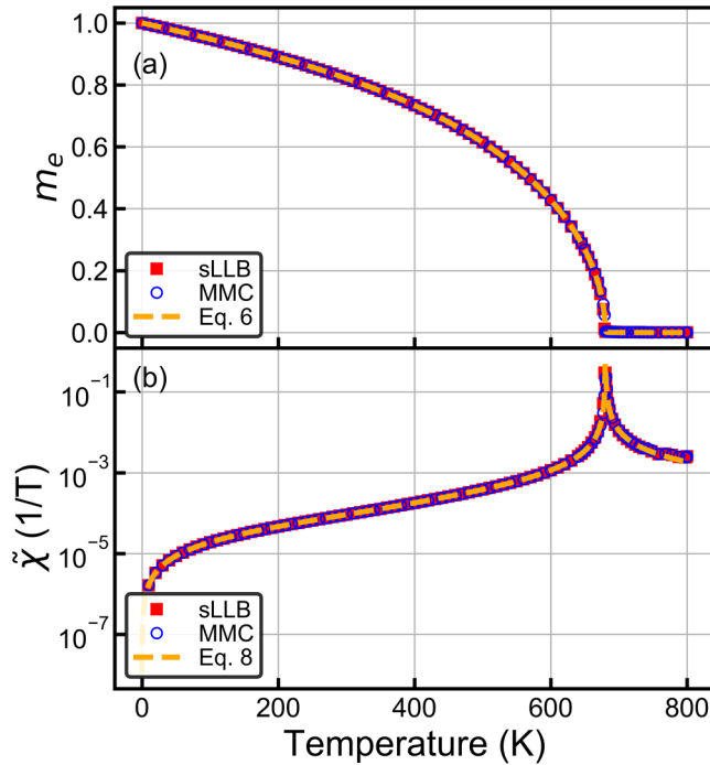
FIG. 2. (a) Normalized equilibrium magnetization length and (b) relative longitudinal susceptibility, computed numerically and compared to model input functions for verification. The distributions produced by MMC and sLLB, respectively, are fitted to obtain m_e and \chi [with Eq. (7) for the longitudinal distribution].
