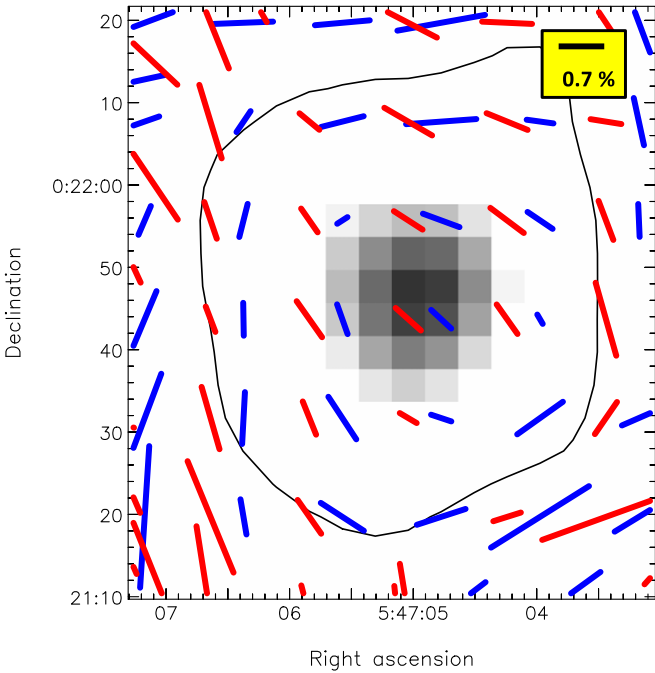
Figure 4. Comparison between 450\ \mu\text{m} (red) and 850\ \mu\text{m} (blue) polarization vectors in the central 60'' \times 70'' area. All polarization vectors are selected using the criterion of (P/\delta P) \geq 3 at both wavelengths. A representative vector with a polarization fraction of 0.7% is shown in the upper right-hand corner. The black contour represents the 450\sigma level of 850\ \mu\text{m} continuum emission, where \sigma = 2.0\ \text{mJy beam}^{-1} .
