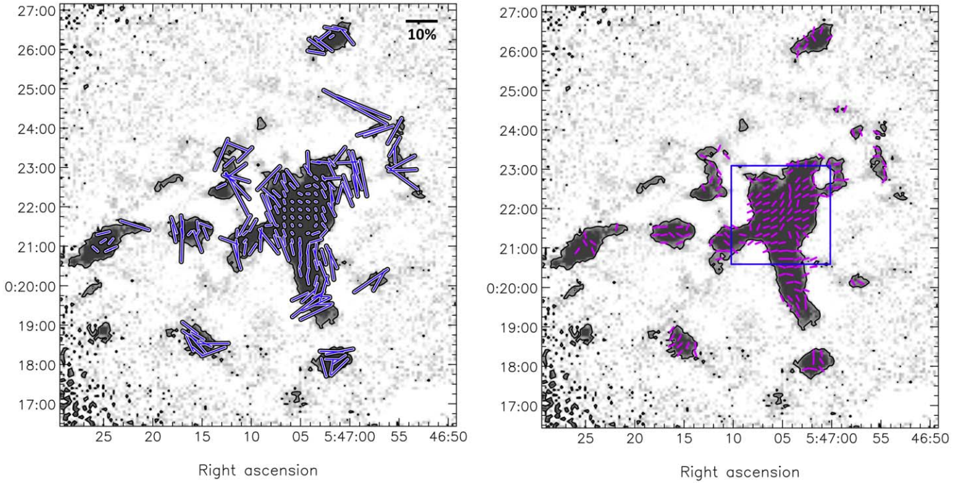
Figure 3. The left-hand panel shows the POL-2 450\ \mu\text{m} polarization vector map. Vectors have a selection criterion of (I/\delta I) \geq 50 and (P/\delta P) \geq 3 . Vector lengths are proportional to their polarization fractions. A representative vector with a polarization fraction of 10% is shown in the upper right-hand corner. The right-hand panel shows the magnetic field vector map, with each 450\ \mu\text{m} polarization vector rotated by 90^\circ . Grayscale represents 450\ \mu\text{m} continuum emission. The black contour corresponds to 20\sigma , where \sigma = 6.5\ \text{mJy beam}^{-1} . The blue box represents the central 2.5 \times 2.5 region, within which an angle dispersion is derived for magnetic field strength measurement using the DCF method.
