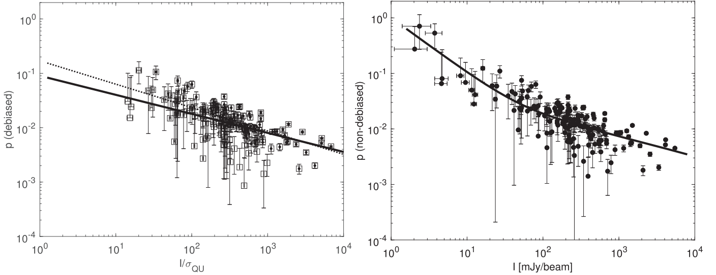
Figure 5. Polarization fraction as a function of total intensity at 850\ \mu\text{m} on 12'' pixels within the central 3' area. The left-hand panel shows a single power-law fit to the debiased polarization fraction as a function of the normalized total intensity with \sigma_{QU} = 0.80\ \text{mJy beam}^{-1} . All squares represent a total of 158 vectors selected using the criterion (I/\delta I) \geq 10 . The obtained power-law slope, \alpha , and P_{\sigma_{QU}} are 0.35 \pm 0.03 and 0.09 \pm 0.02 (solid line), respectively. Filled circles represent a total of 96 vectors, selected using the criterion (P/\delta P) \geq 3 . The obtained power-law slope, \alpha , and P_{\sigma_{QU}} are 0.43 \pm 0.04 and 0.17 \pm 0.05 (dotted line), respectively. The right-hand panel shows the Rician fitting to the nonbiased polarization fraction as a function of the total intensity for the whole data set within the central 3' region. The derived \alpha and P_{\sigma_{QU}} are 0.36 \pm 0.04 and 0.10 \pm 0.03 , respectively (see details about Rician fitting in Pattle et al. 2019). We note that negative error bars for some data points are not shown due to the logarithmic scale of the vertical axis. Some error bars are too small to be seen compared to the symbol size.
