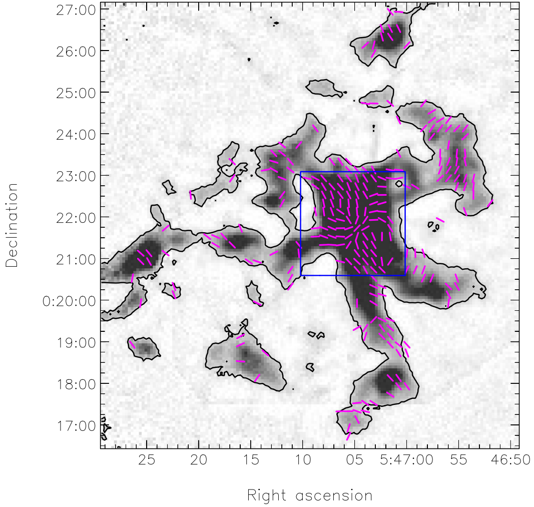
Figure 2. Magnetic field vector map, with each 850 \mu\text{m} polarization vector rotated by 90°, of NGC 2071IR. Vectors are selected using the criteria (I/\delta I) \geq 10 and (P/\delta P) \geq 3 . Black contours correspond to 10\sigma , where \sigma = 2.6 \text{ mJy beam}^{-1} . The blue box represents the central 2.5 \times 2.5 region, within which an angle dispersion is derived for magnetic field strength measurement using the DCF method.
