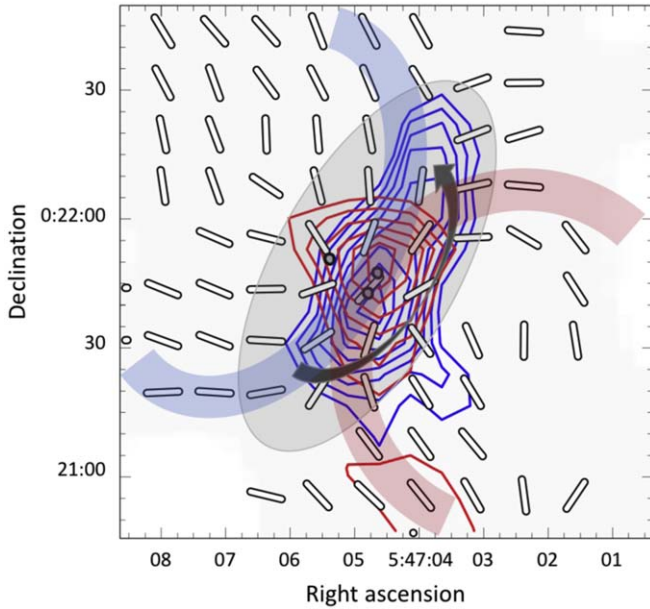
Figure 9. Magnetic field vectors derived from 850 \mu\text{m} polarization data using selection criteria of (I/\delta I) \geq 10 and (P/\delta P) \geq 3 . The blue and red contours, which are the same as those in Figure 8, represent the HARP \text{C}^{18}\text{O} (3–2) emission. We overlay a cartoon showing our suggestion of a rotating disklike structure and outflow. The shaded blue and red colors schematically represent outflow cavity walls, and the shaded gray color represents a disklike structure.
