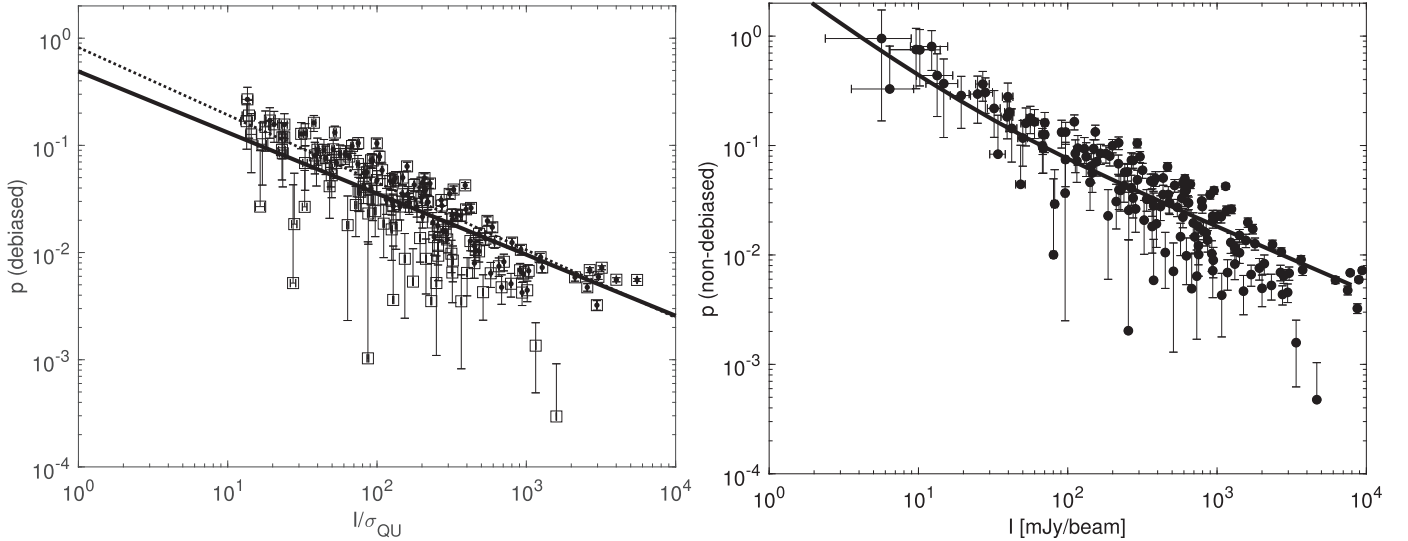
Figure 6. Polarization fraction as a function of total intensity at 450\ \mu\text{m} on 12'' pixels within the central 3' area. The left-hand panel shows a single power-law fit to the debiased polarization fraction as a function of the normalized total intensity with \sigma_{QU} = 2.93\ \text{mJy beam}^{-1} . All squares represent a total of 150 vectors selected using the criterion (I/\delta I) \geq 10 . The obtained power-law slope, \alpha , and P_{\sigma_{QU}} are 0.57 \pm 0.03 and 0.49 \pm 0.11 (solid line), respectively. Filled circles represent a total of 105 vectors, selected using the criterion (P/\delta P) \geq 3 . The obtained power-law slope, \alpha , and P_{\sigma_{QU}} are 0.63 \pm 0.03 and 0.82 \pm 0.17 (dotted line), respectively. The right-hand panel shows the Rician fitting to the nonbiased polarization fraction as a function of the total intensity for the whole data set within the central 3' region. The derived \alpha and P_{\sigma_{QU}} are 0.59 \pm 0.03 and 0.55 \pm 0.12 , respectively. We note that negative error bars for some data points are not shown due to the logarithmic scale of the vertical axis. Some error bars are too small to be seen compared to the symbol size.
