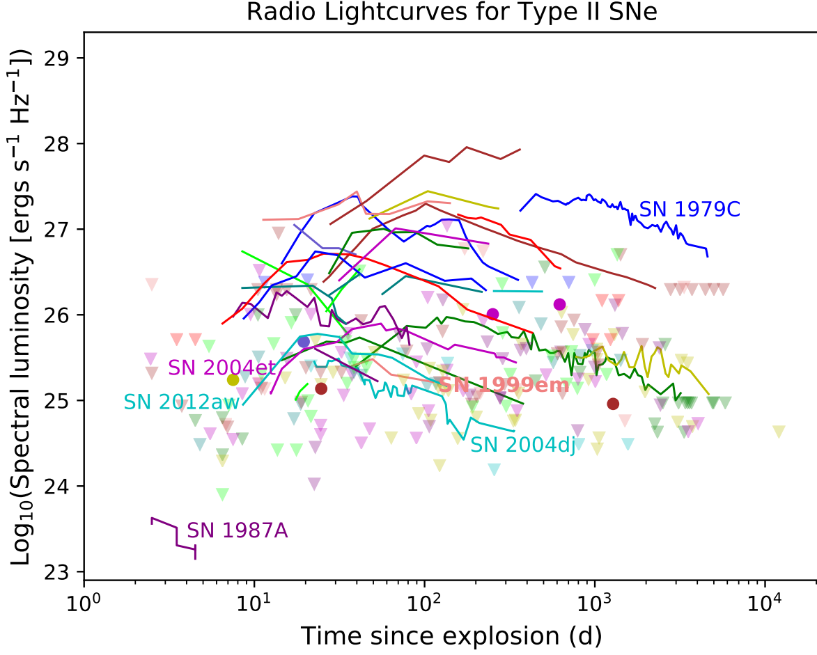
Figure 4. As Figure 2, but showing only the 106 SNe of Type II (excluding Type IIn) at D < 100 Mpc. Different colors are used for the different SNe. The lightcurves for several SNe, including SN 1987A, are labeled in the corresponding colors. The lightcurve for SN 1987A is at 2.3 GHz, unlike all the others which are at 4 to 10 GHz.
