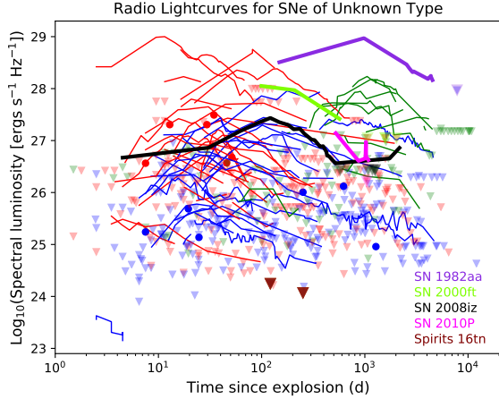
Figure 15. The radio lightcurves or limits of five SNe which were not spectroscopically identified, compared to those of the spectroscopically confirmed SNe of Types I b/c (red) and II (blue) and IIn (green) in our sample. SNe 1982aa, 2000ft, 2008iz, 2010P and Spirits 16tn are highlighted in violet, light green, black, magenta and maroon, respectively. Spirits 16tn was not detected, but two fairly low limits were obtained, shown as larger maroon triangles between t = 100 and 300 d. SN 1982aa is most likely of Type IIn. For SNe 2000ft, 2008iz and 2010P, and Spirits 16tn, the radio lightcurves do not permit a conclusive identification of the SN Type.
