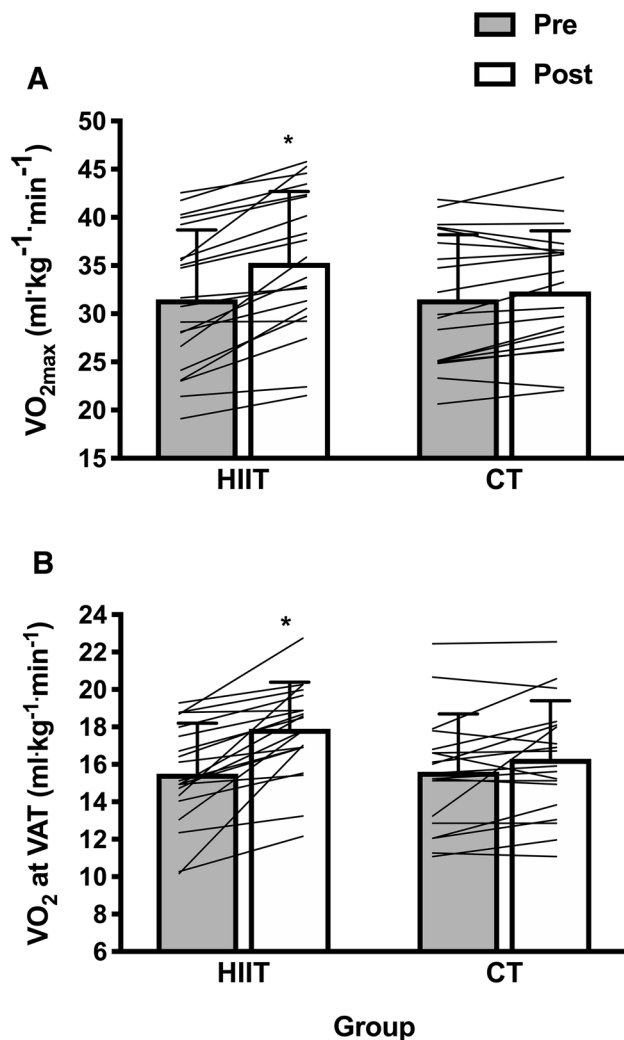
Fig. 2 Maximal oxygen consumption ( \dot{V}O_{2\max} ) (a) and \Delta after 8 weeks of HIIT ( n=20 ) and CT ( n=19 ). Black lines correspond to individual responses. \dot{V}O_2 oxygen uptake, VAT ventilatory anaerobic threshold, HIIT low-volume high-intensity interval training, CT circuit training. * P < 0.001 versus baseline
