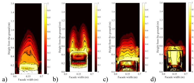
Fig. 6. Intermittency contours for a) BC30W50xH25, b) BC30W50xH50, c) FR30W50xH25, d) FR30W50xH50.
