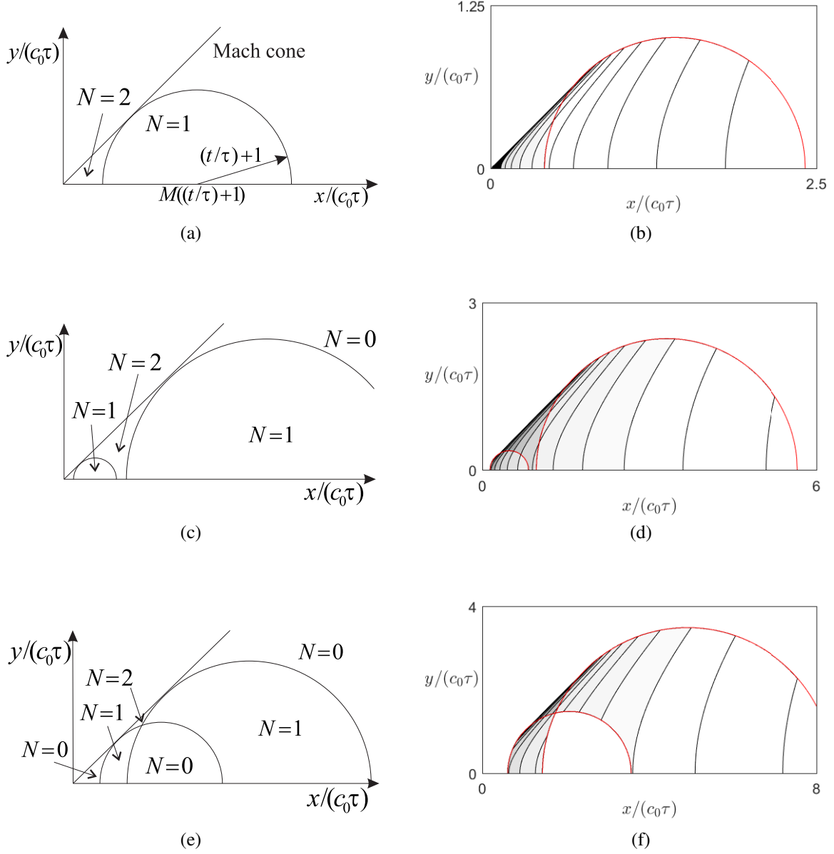
Figure 2: Development in time of the pressure field generated by a gust with spanwise delta-function and streamwise top-hat profile, convected at Mach number M = \sqrt{2} . On the left are wavefronts and corresponding values of N ; on the right are contours of the pressure field scaled by \rho_0 M c_0 \bar{v}_0 , together with the wavefronts marked in red. The pressure is negative or zero everywhere, and the most negative pressures are indicated by the darkest shading. Across the wavefronts, the pressure field is discontinuous. In (a–b), for t/\tau = 0 , the gust is still striking the leading edge; in (c–d), for t/\tau = 0.95M , the gust has just passed the leading edge; and in (e–f), for t/\tau = 1.75M , the initial and final wavefronts have overlapped, leaving an interior silent region. The plots are obtained from Eqn. (12).
