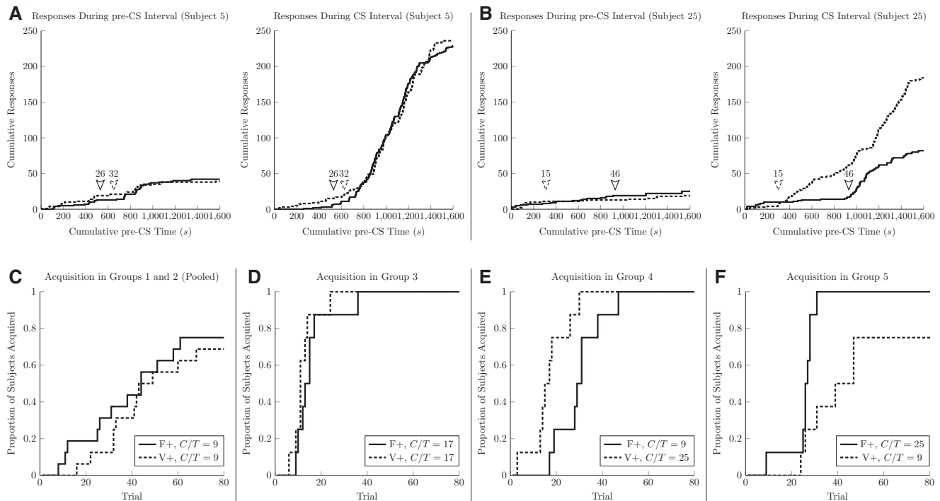
Figure 3. Change-point analysis for the acquisition of conditioned responding. (A) Cumulative responses for a representative subject in Group 1 during the pre-CS interval of the ITI (left) and the CS presentation (right) for Fixed+ trials (solid line) and Variable+ trials (dashed line). The arrows indicate the point identified by the change-point analysis to be the likely point of acquisition. (B) An identical plot to that in A, showing results for a representative subject in Group 4, when F+ and V+ were expected to be learned at different times. (C–F) Cumulative plots showing the proportion of subjects who had acquired by a given trial. Given their similarity, Groups 1 and 2 were pooled in C.
