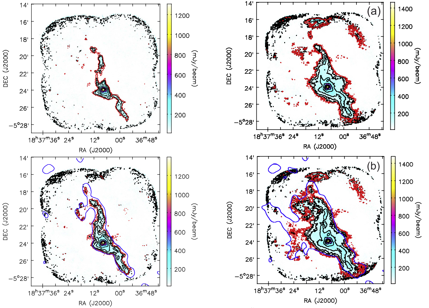
Figure 24. Top panel: SCUBA-2 850 \mu\text{m} continuum emission in the R1 data reduction for G26. The contour levels are [0.03, 0.05, 0.1, 0.2, 0.4, 0.6, 0.8] \times 1.35 \text{ Jy beam}^{-1} . Bottom panel: SCUBA-2 850 \mu\text{m} continuum emission in the R2 data reduction. The contour levels are [0.03, 0.05, 0.1, 0.2, 0.4, 0.6, 0.8] \times 1.40 \text{ Jy beam}^{-1} . The red contour in both panels shows the S/N level of 3.
