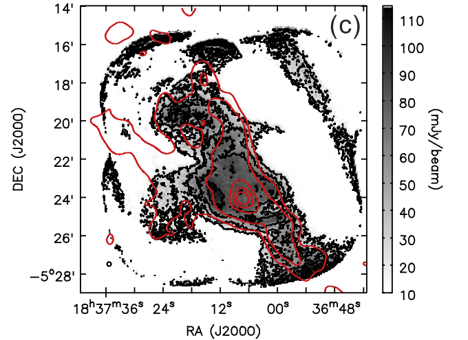
Figure 25. (a) SCUBA-2 850 \mu\text{m} continuum emission in the R3 data reduction, shown in color scale and black contours. The contour levels are [0.03, 0.05, 0.1, 0.2, 0.4, 0.6, 0.8] \times 1.47 \text{ Jy beam}^{-1} . The red contour shows the S/N level of 3. (b) SCUBA-2 850 \mu\text{m} continuum emission in the R4 data reduction, shown in color scale and black contours. The contour levels are [0.03, 0.05, 0.1, 0.2, 0.4, 0.6, 0.8] \times 1.48 \text{ Jy beam}^{-1} . The red contour shows the S/N level of 3. The blue contour outlines the external mask from the Herschel column density map. (c) Extended SCUBA-2 850 \mu\text{m} continuum emission ( R4 – R2 ), shown in gray scale and black contours. The contour levels are [0.2, 0.4, 0.6, 0.8] \times 0.11 \text{ Jy beam}^{-1} . The red contours show the column density derived from Herschel /SPIRE data. The contour levels are [0.15, 0.2, 0.4, 0.6, 0.8] \times 4.8 \times 10^{22} \text{ cm}^{-2} .
