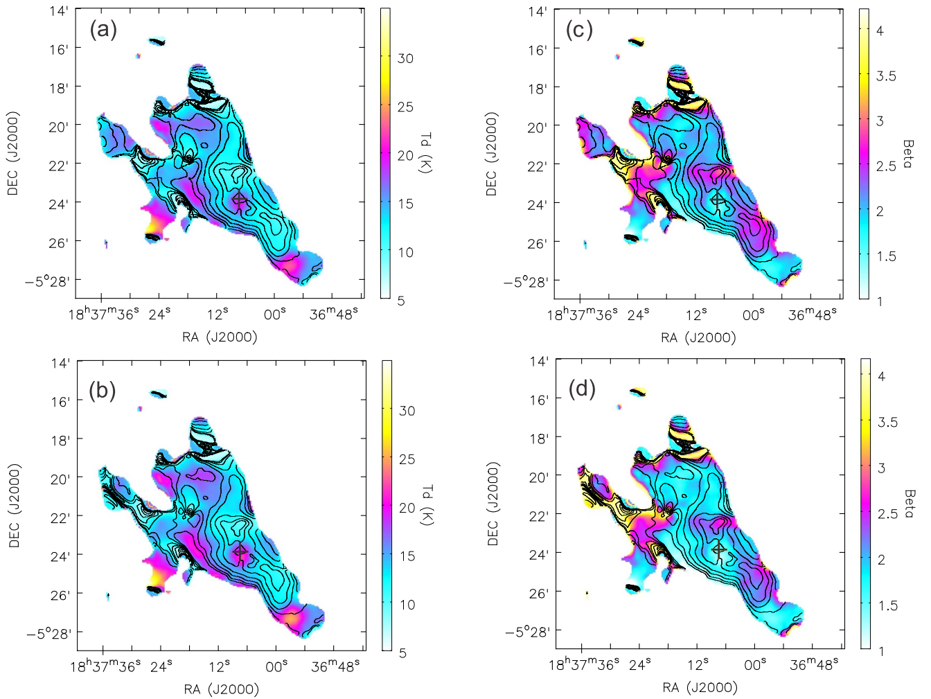
Figure 7. (a) Dust temperature map in the SED fit with free \beta using the Herschel data only shown in color scale. The 250\ \mu\text{m} optical depth is shown with contours. The contour levels are [0.03, 0.05, 0.1, 0.2, 0.4, 0.6, 0.8] \times 0.0282 . (b) Dust temperature map in the SED fit with free \beta using both the Herschel and SCUBA-2 data shown in color scale. The 250\ \mu\text{m} optical depth is shown with contours. The contour levels are [0.03, 0.05, 0.1, 0.2, 0.4, 0.6, 0.8] \times 0.0211 . (c) \beta map in the SED fit with free \beta using the Herschel data only, shown in color scale. The 250\ \mu\text{m} optical depth is shown with contours. The contour levels are the same as in panel (a). (d) \beta map in the SED fit with free \beta using both the Herschel and SCUBA-2 data shown in color scale. The 250\ \mu\text{m} optical depth is shown with contours. The contour levels are the same as in panel (b). The plus signs in the four panels mark the position of the most massive clump.
