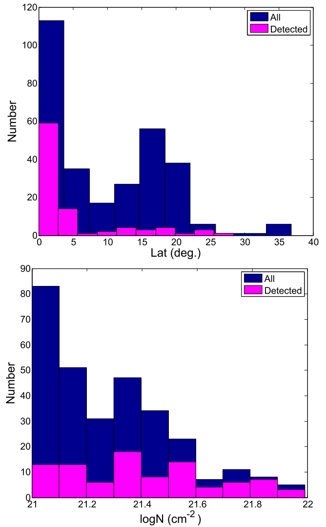
Figure 3. SCUBA-2 detections as a function of latitude (top panel) and column density (bottom panel) for PGCCs in the pilot study. The 300 PGCCs in pilot studies are shown in blue, while those with SCUBA-2 detections are shown in pink.
