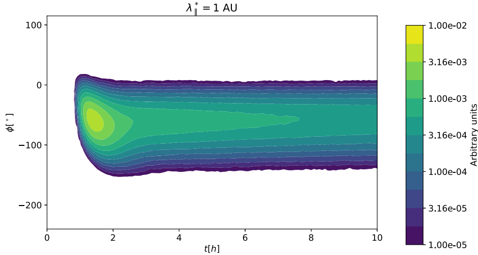
Fig. 5. 10 MeV SEP intensity at 1 AU, as a function of time and heliographic longitude, with magnetic connection along the Parker spiral at \varphi = -62^\circ , for \lambda_{||}^* = 1 AU.
