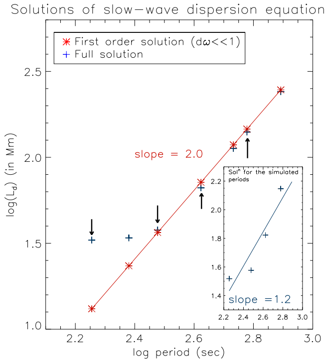
Figure 8. Log-log plot of damping lengths obtained by solving the Equation (2) for a range of periods (3–13 minutes). The red (*) represent first-order solutions corresponding to the lower thermal conduction limit ( d\omega \ll 1 ), whereas the blue (+) symbols represent the full solutions. The obtained slope for the first-order solutions (represented by a red line) is equal to 2, whereas the slope for the full solutions for the frequencies used in the simulation is equal to 1.2 (as shown in the blue line in the inset plot).
