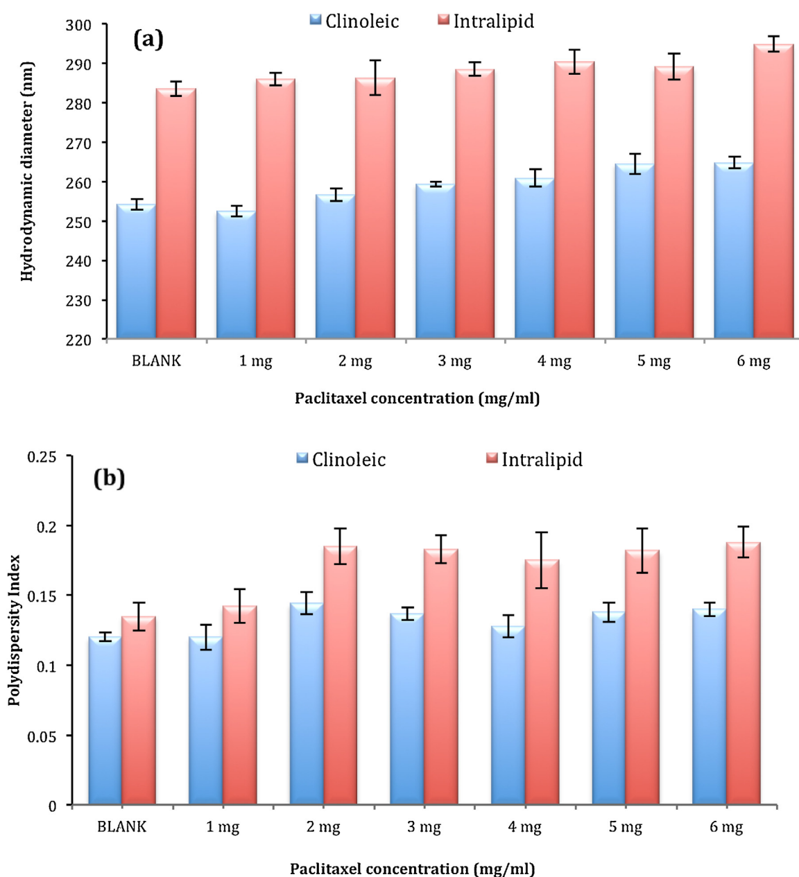
Fig. 1. (a) Size (Zaverage) and (b) PI of Clinoleic and Intralipid nanoemulsion droplets at a range of paclitaxel concentrations ( n = 3 \pm \text{SD} ).
