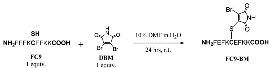
Figure 2. Scheme of the synthetic route used to produce FC9-BM peptide.
