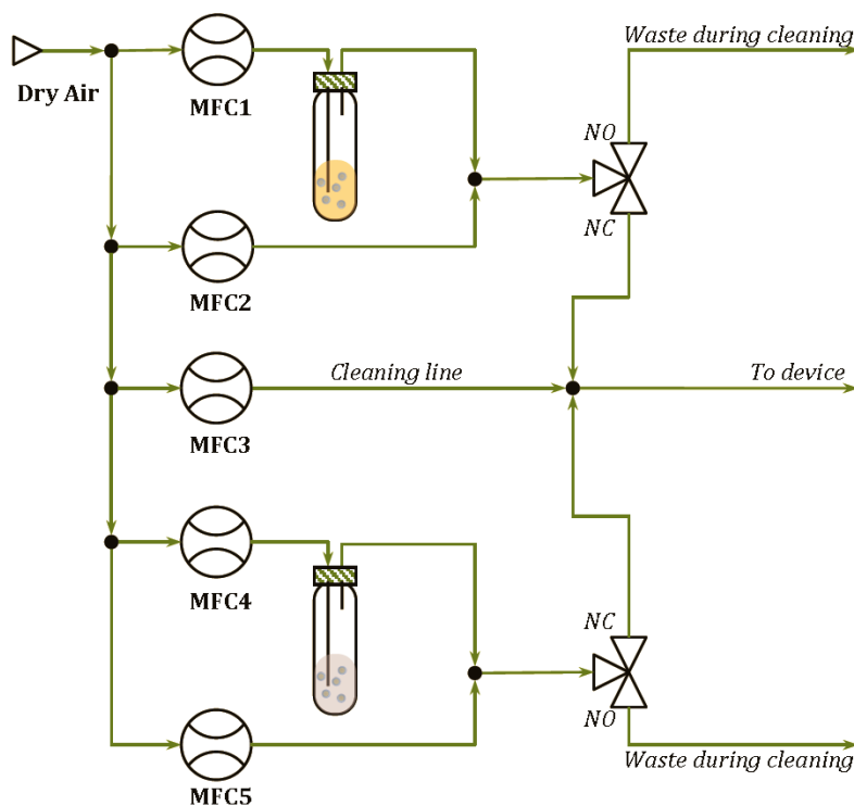
Figure 3. System set up for delivering binary mixtures.
