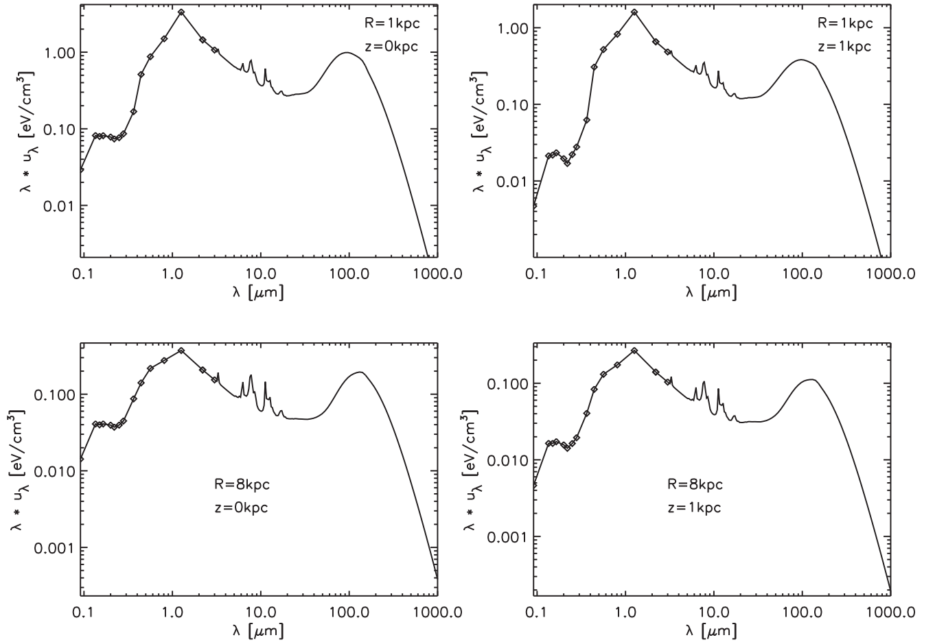
Figure 9. SEDs of RFs at various galactocentric positions. The symbols are for the UV/optical wavelengths at which the RT calculations were performed. For the dust emission, the calculations were performed at 500 wavelengths, logarithmically spaced.
