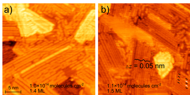
FIG. 3. 30 nm \times 30 nm topographs of the Pn/Cu/AIPdMn surface. (a) I_T = 150 pA, V_B = 1.6 V. Checkerboard structure has been almost completely replaced by another row structure. Noise is observed around some molecules in the remaining checkerboard structure, indicating that these molecules have become unstable in this adsorption configuration. (b) I_T = 110 pA, V_B = 1.05 V. Slightly higher coverage. No checkerboard Pn remains. The differing heights of the Pn rows shown in the profile are likely to be evidence of tilted rows as explained in the text. \Delta z given is between the tops of adjacent rows and does not include the Pn layer thickness. In the lower right portion of the image, a transition between 4 flat rows and 3 flat + 2 tilted rows in the same cross-rows distance is indicated. An additional example is shown in the upper middle portion, where 3 flat rows have a small section with an additional tilted row inserted.
