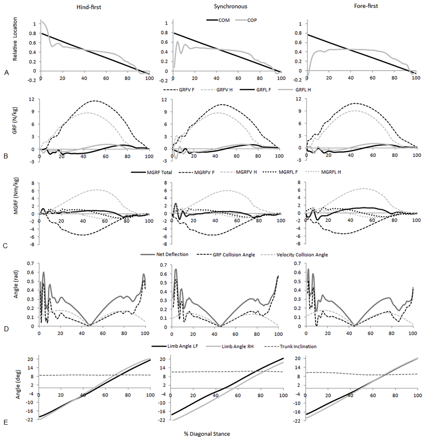
Figure 3 Examples of significant parameters from typical hind-first, synchronous and fore-first dissociation patterns when speed-matched. (A) Relative COM and COP location from the forelimb COP position at Tzero; (B) Vertical (GRFV) and longitudinal (GRFL) GRFs for the fore and hindlimbs (N/kg); (C) total and fore and hindlimb components of ground reaction force moments (MGRF) (Nm/kg); (D) GRF collision angle, velocity collision angle and net deflection (rad); (E) Fore and hindlimb angles and trunk inclination (degrees).
