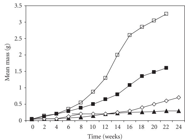
FIGURE 7: Typical earthworm growth curves obtained from periodic measurement of masses. Here Lumbricus terrestris was examined under constant temperature conditions (□ – 20; ■ – 15; ◇ – 10; ▲ – 5°C; adapted from [44]).
