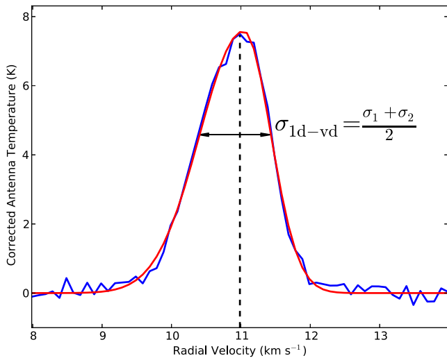
Figure 2. \text{C}^{18}\text{O} , J = 3\text{--}2 line emission (blue) and skew-Gaussian fit (red) at a pixel within Filament 26. The variables \sigma_1 and \sigma_2 are the Gaussian standard deviations either side of the central peak which are averaged to provide a more accurate estimate of the velocity dispersion when the emission line profile is asymmetric.
