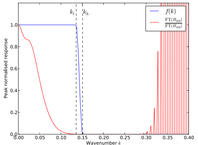
Figure 6. The one-dimensional slice through the filter response and peak normalized \frac{FT(B_{850})}{FT(B_{450})} . It is clear that the choice of k_h removes the contribution of high-frequency noise ( k > 0.3 ) produced by division of extremely small values present in the Fourier transforms of the 450 and 850 \mu\text{m} beam profiles.
