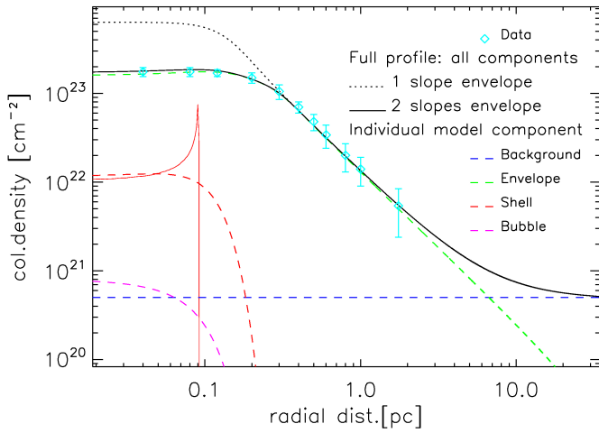
Fig. 7. Column density profile of the central UCH II region (cyan diamonds with \sigma errors bars) compared to models with all components illustrated in Fig. 3. The neutral envelope with two density gradients or with a single one are shown by a black line and a dotted black line respectively. An envelope model with a single density gradient cannot match the observed data. Individual components after convolution by the beam are shown by magenta, red, green, and blue dashed lines, for the bubble, shell, envelope and background. The continuous red line shows the unconvolved shell profile at an infinite resolution.
