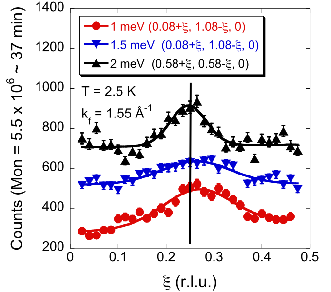
FIG. 5. Constant-energy scans across the q-1D excitation in the x = 0.45 sample measured at 1.0, 1.5 (scan B), and 2 meV (scan A). The solid lines are the result of a fit to the data of a sloping background with one Gaussian line shape. The wave vector resolution parallel to the scan resolution is 0.0124 r.l.u. at 1.0 meV, 0.0127 r.l.u. at 1.5 meV, and 0.0131 r.l.u. at 2 meV. A broadening of the q-1D excitation is observed in scans at 1.0 and 1.5 meV, compared to 2 meV.
