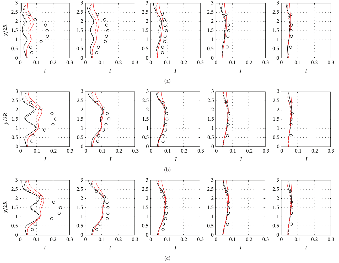
FIGURE 8: Turbulence intensity at 8R, 14R, 22R, 30R, and 40R downstream of the disc, with the channel (solid line), duct (dashed line), and experimental data (○) [11] at different C_T values of (a) 0.61, 0.62, (b) 0.86, 0.91, and (c) 0.97, 0.99 for this study and the experiment study, respectively [11]. The inlet 1 simulations are shown in black and inlet 2 simulations are in red.
