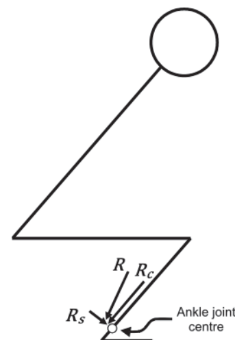
Figure 6: Computation of R_c and R_s at the ankle joint 16,21,22
