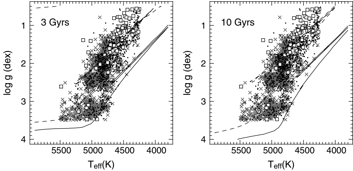
Fig. 1. \log g versus T_{\text{eff}} values for the SN75 RAVE sample (see text) with overplotted isochrones of 3 Gyr (left panel) and 10 Gyr (right panel) with metallicities [M/H] = 0.0 dex (solid lines) and [M/H] = -1.0 dex (dashed lines). Black points, grey crosses, and open squares represent the thin disc, dissipative, and accretion components as defined in Sect. 4.
