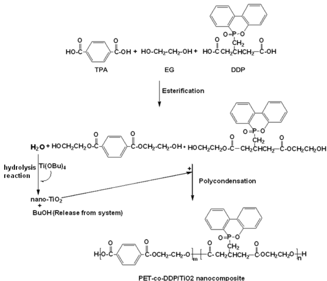
Scheme 1 The single-step synthesis of fire retardant PET/TiO 2 nanocomposite
