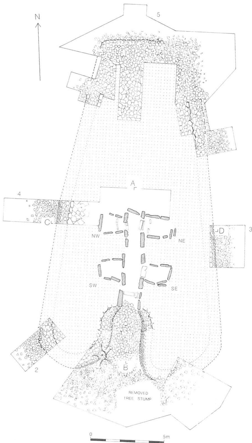
Fig. 2 Excavation plan 1960-61
