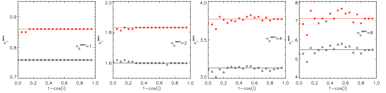
Fig. 5. Derived Sérsic index n_i^{\text{sers}} of the dust-free images of the bulge for bulges produced with volume stellar emissivities described by (de-projected) Sérsic functions with different Sérsic indices. The symbols represent the measurements while the solid line are polynomial fits to the measurements. From left to right , the plots correspond to the bulge Sérsic index values n_0^{\text{sers}} = 1.0, 2.0, 4.0 , and 8.0 . The black curves correspond to bulges truncated at three effective radii while the red curves denote bulges truncated at ten effective radii.
